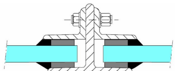
Wet sealing with compatible sealing product
