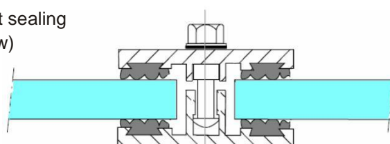
Dry sealing with compatible gasket
